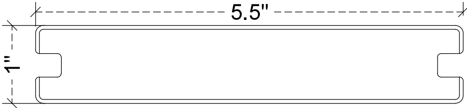
GROOVED DECK BOARD
